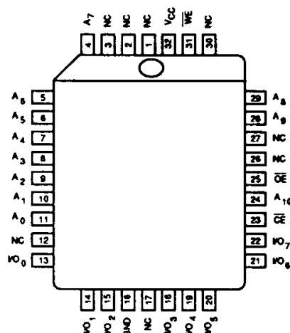
PLASTIC LEADED CHIP CARRIER TOP VIEW
